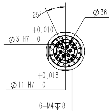
Flange Installation Diagram
