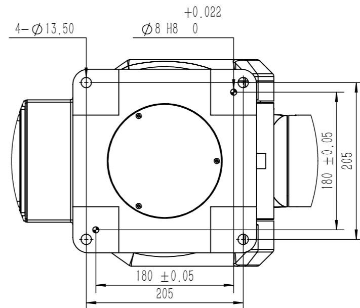
Base Installation Diagram
